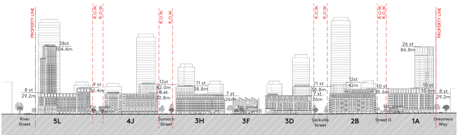
Site Elevation 2 - Gerrard Street East
